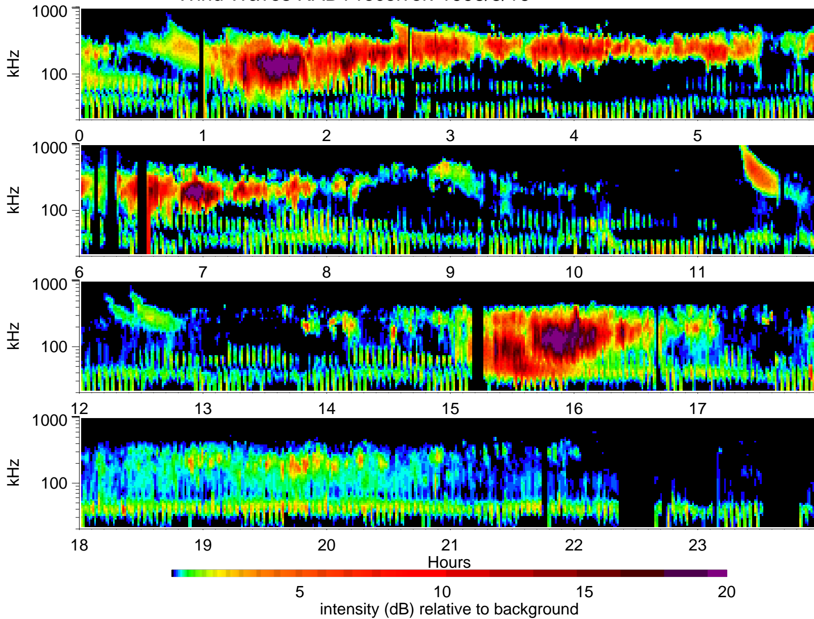
Wind Waves RAD1 receiver: 1998/3/16
