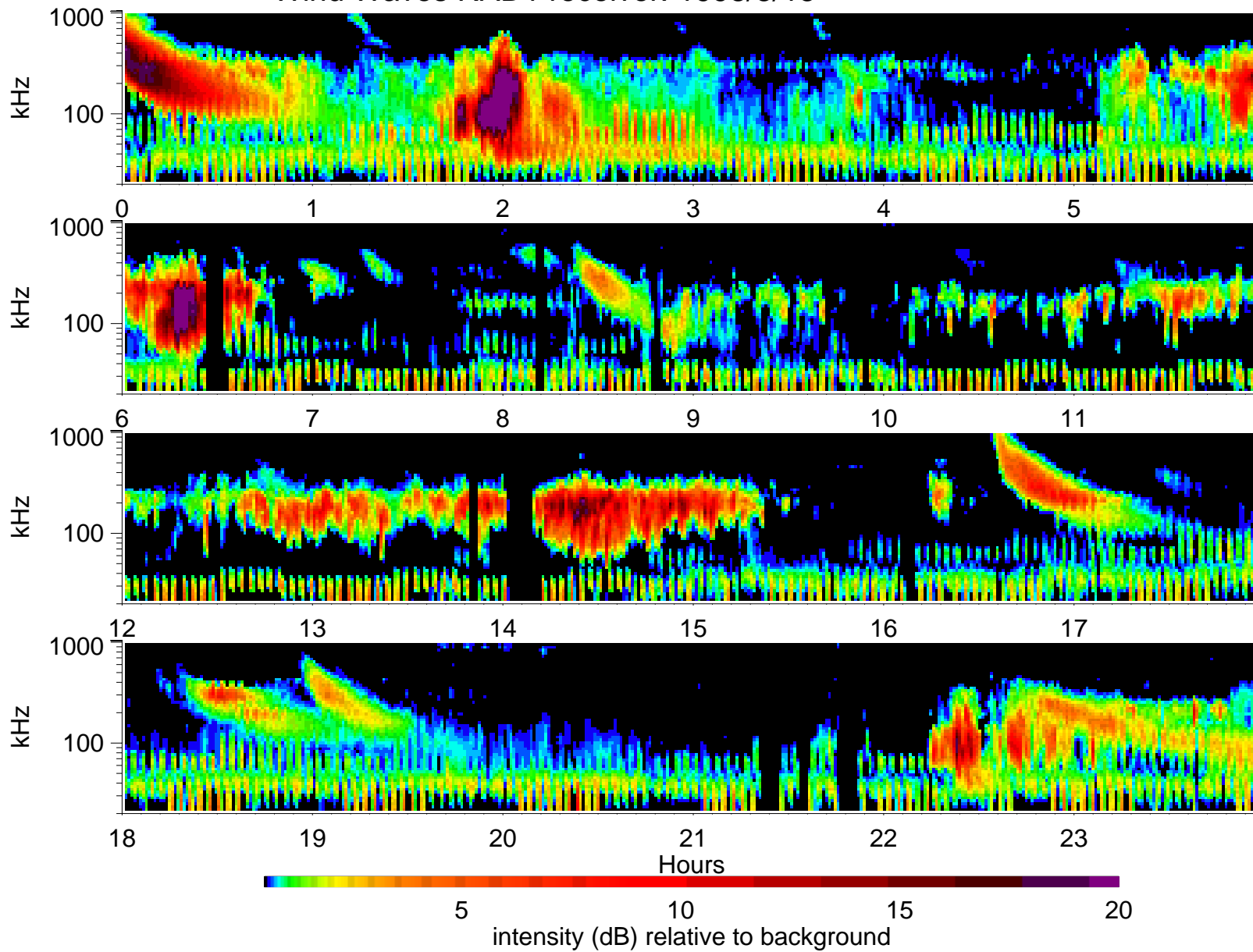
Wind Waves RAD1 receiver: 1998/3/15
