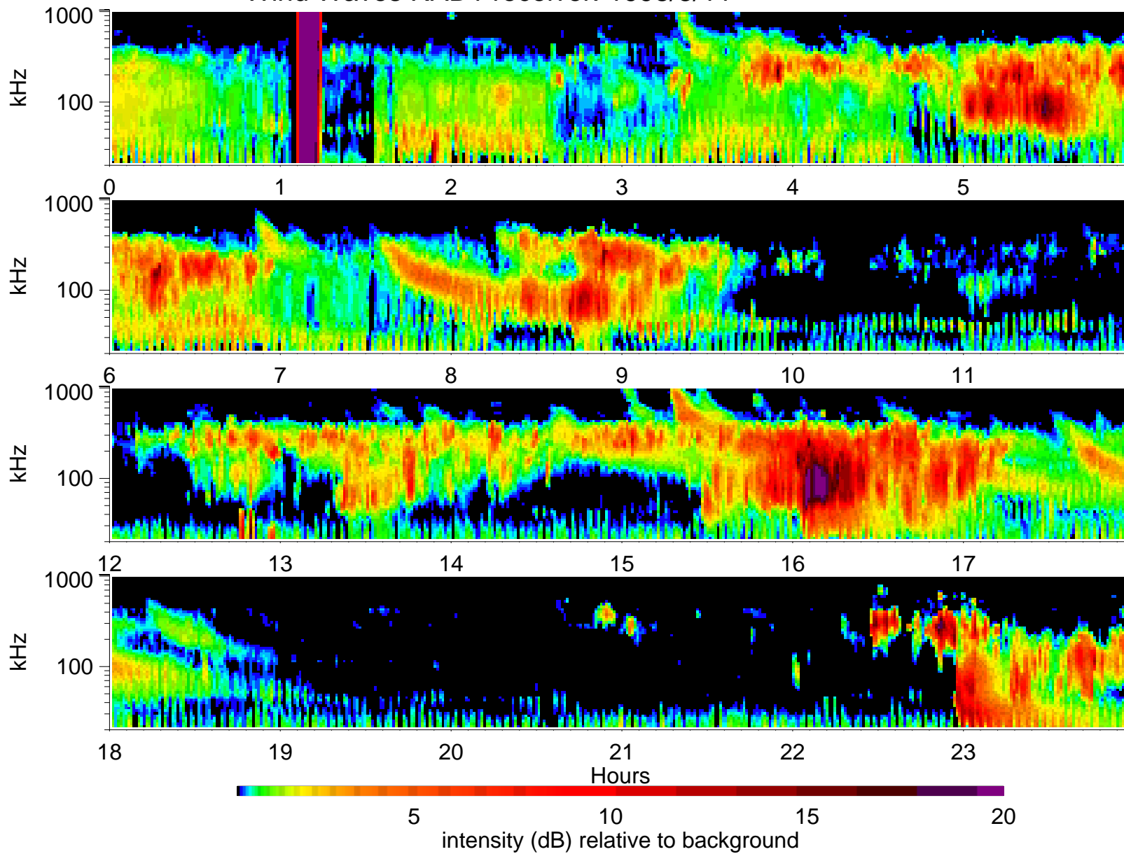
Wind Waves RAD1 receiver: 1998/3/11
