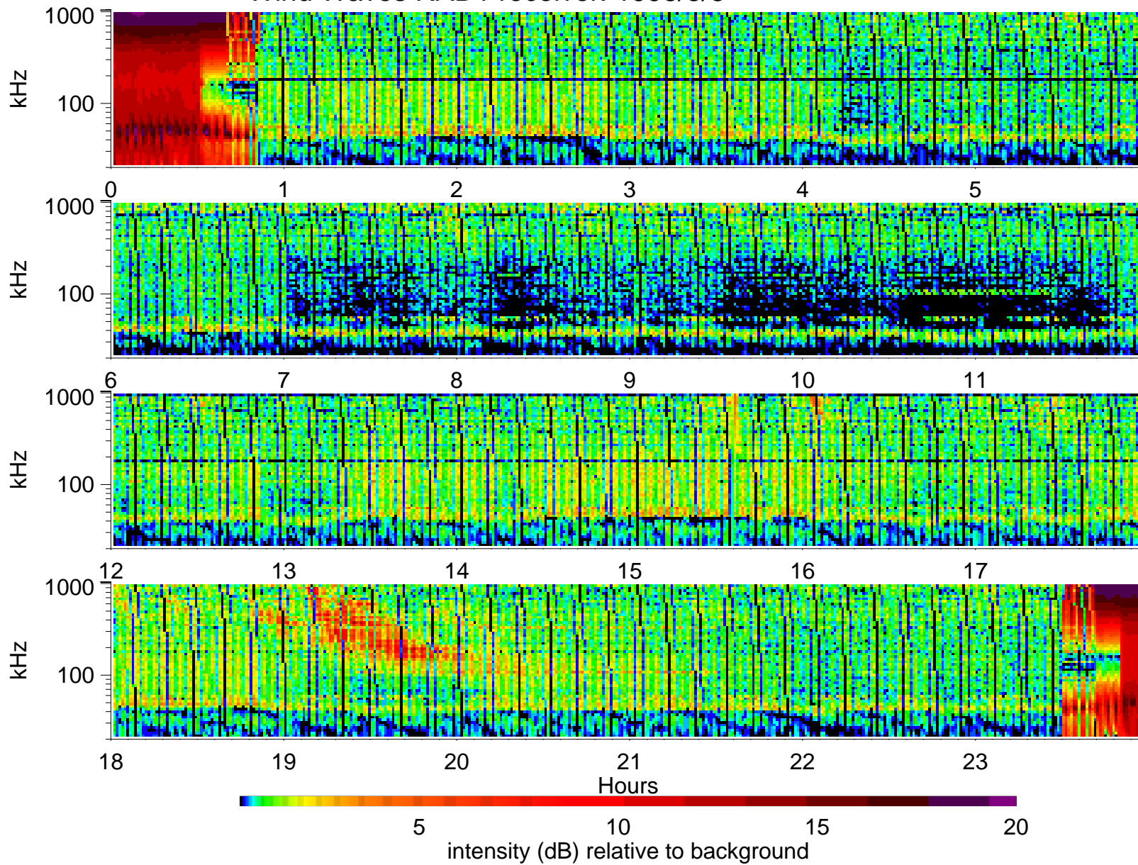
Wind Waves RAD1 receiver: 1998/3/8
