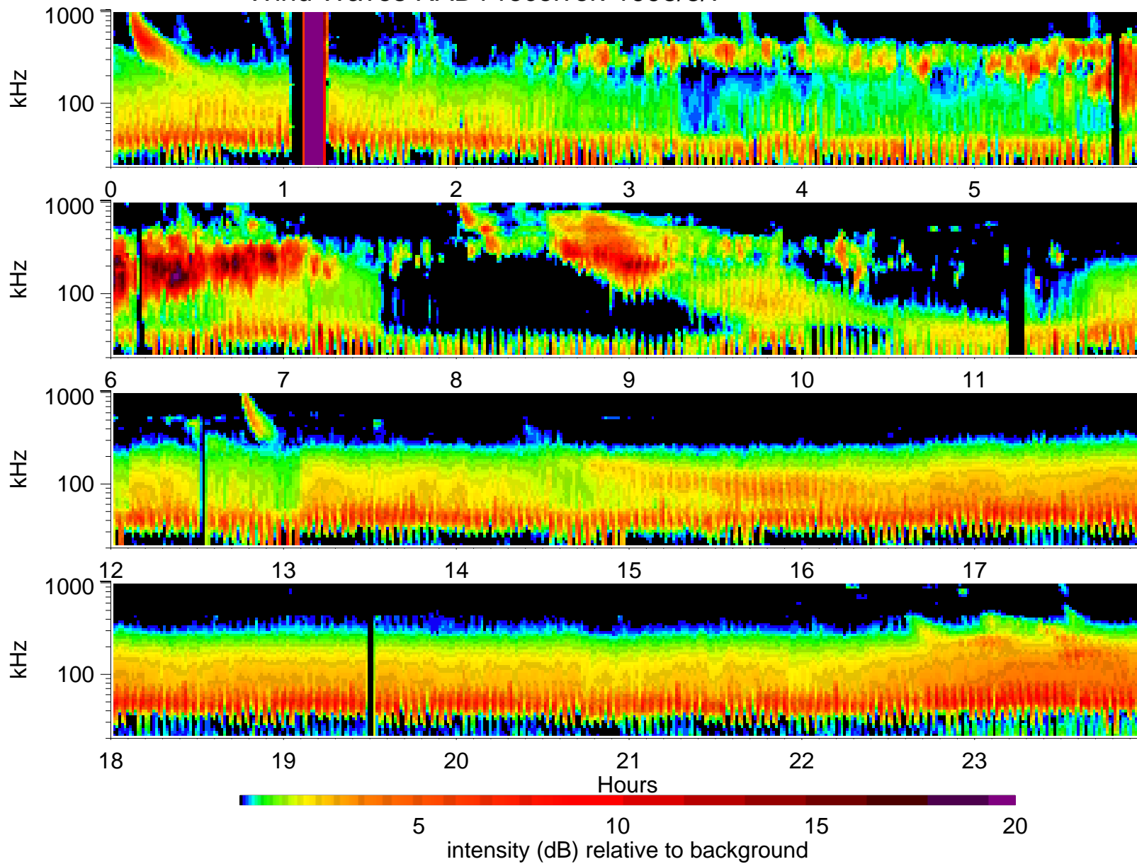
Wind Waves RAD1 receiver: 1998/3/7
