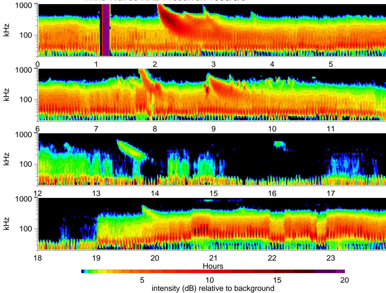
Wind Waves RAD1 receiver: 1998/3/5
