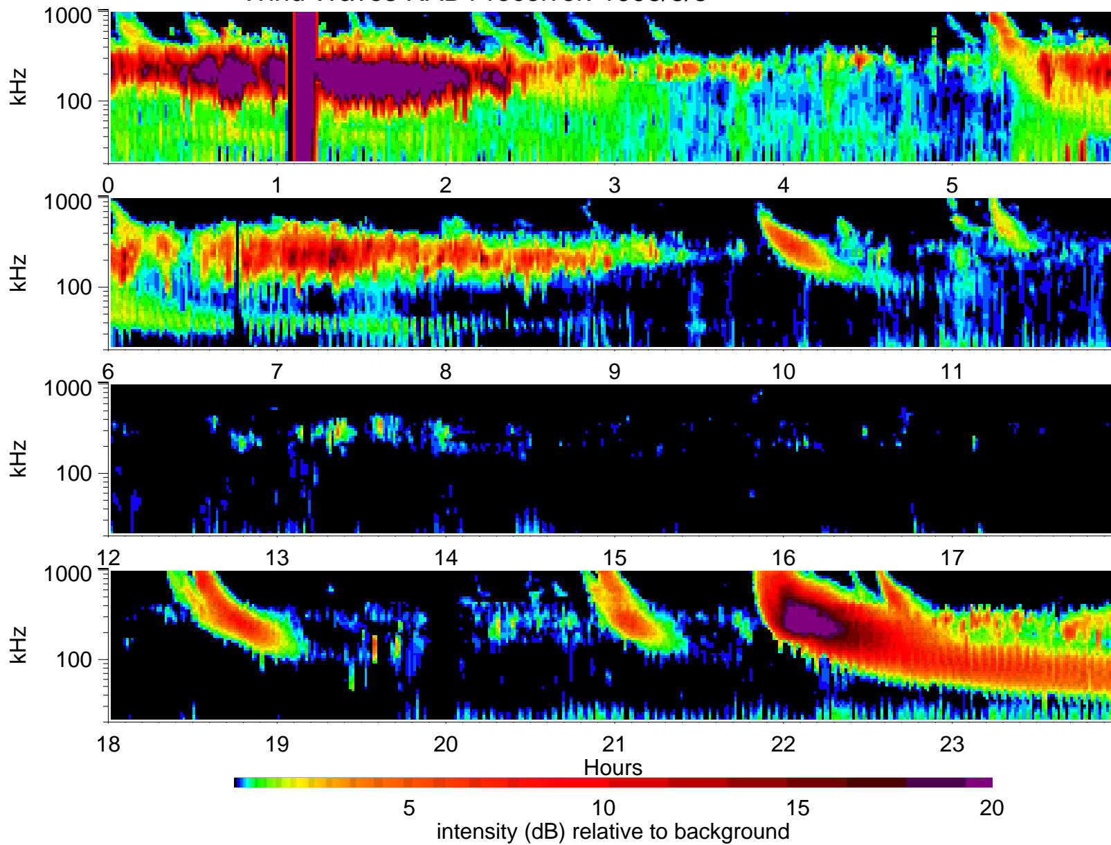
Wind Waves RAD1 receiver: 1998/3/3
