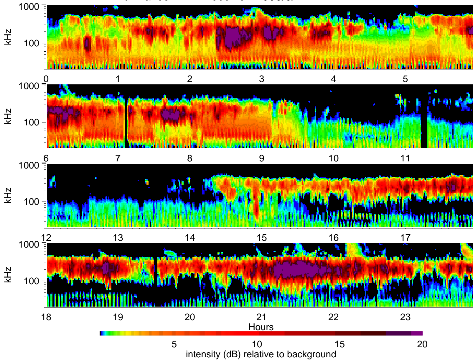
Wind Waves RAD1 receiver: 1998/3/2
