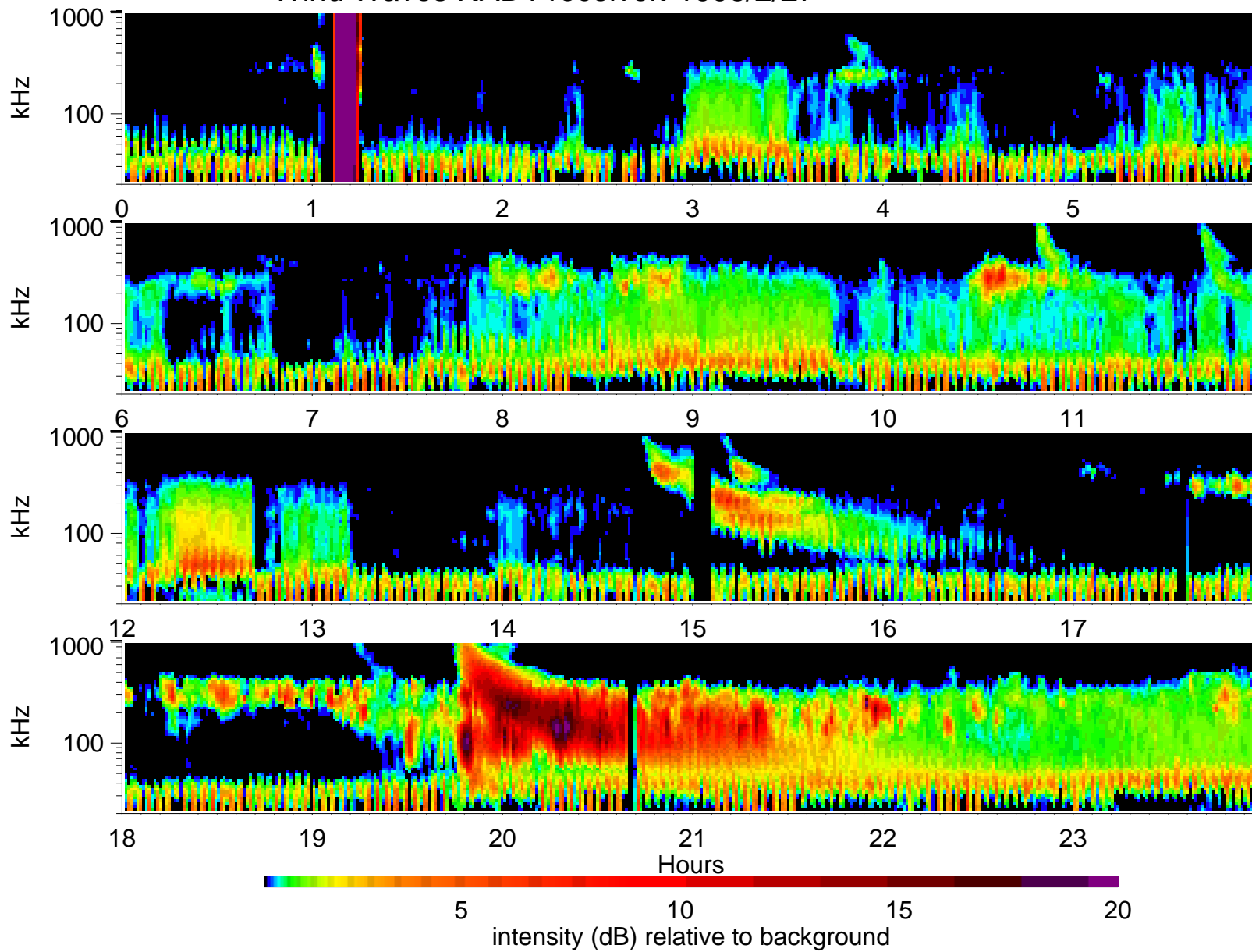
Wind Waves RAD1 receiver: 1998/2/27
