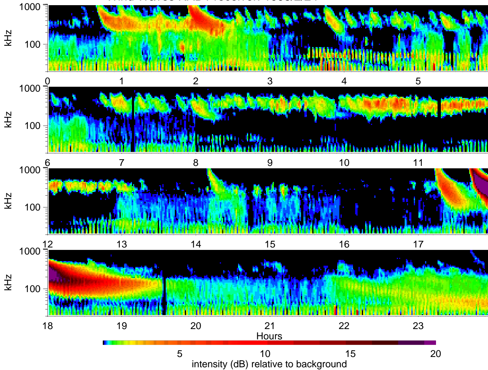
Wind Waves RAD1 receiver: 1998/2/24
