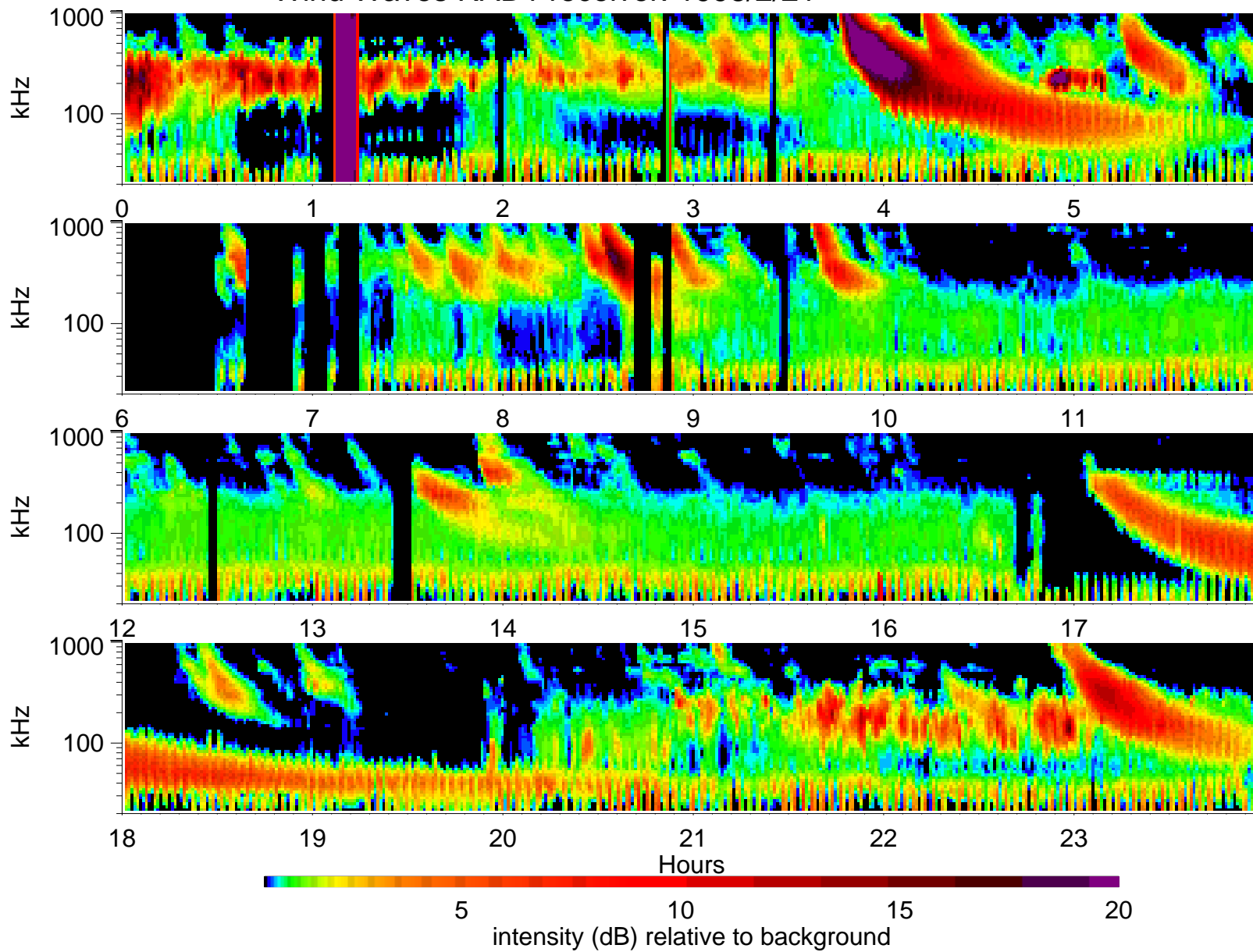
Wind Waves RAD1 receiver: 1998/2/21
