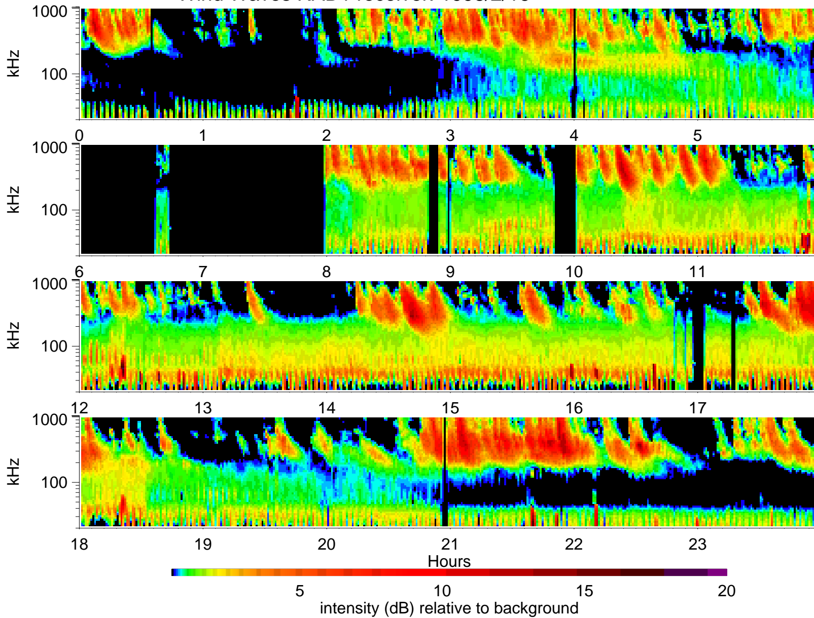
Wind Waves RAD1 receiver: 1998/2/16
