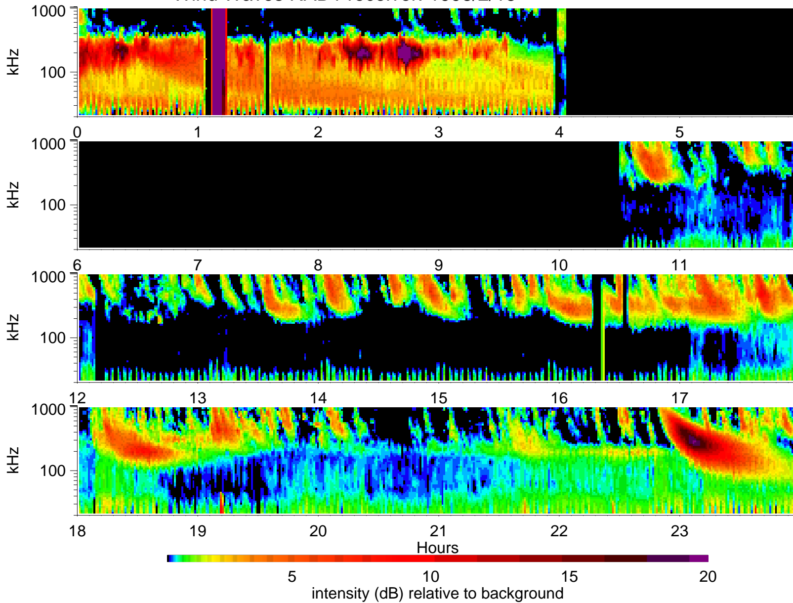
Wind Waves RAD1 receiver: 1998/2/15
