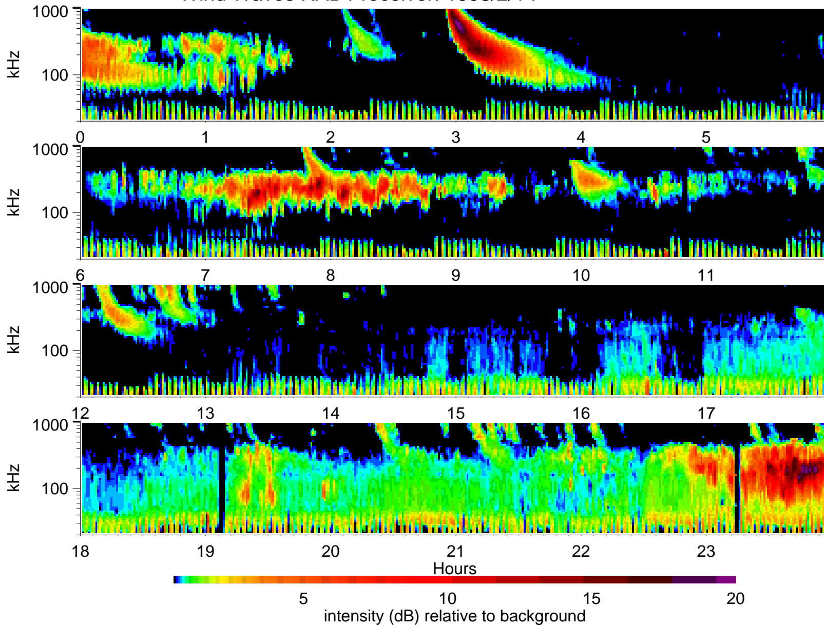
Wind Waves RAD1 receiver: 1998/2/14
