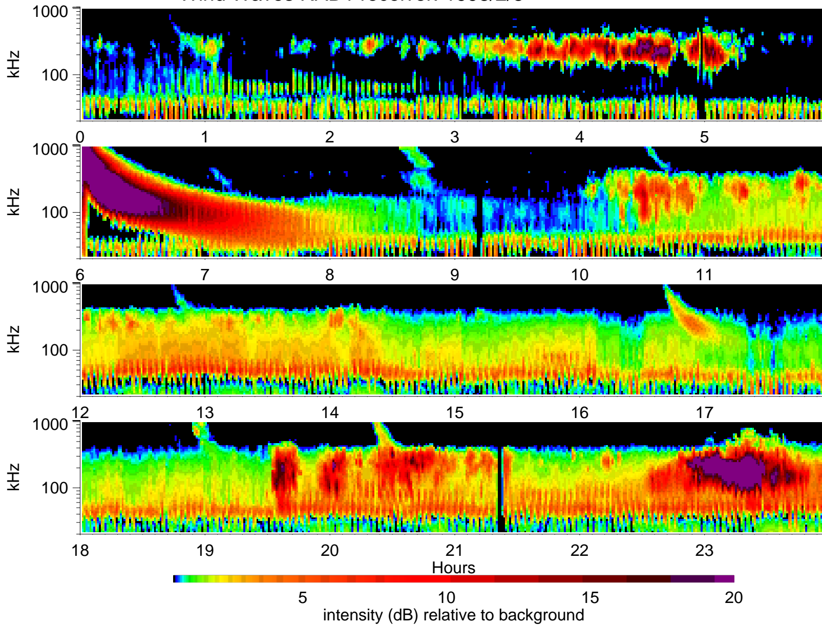
Wind Waves RAD1 receiver: 1998/2/8
