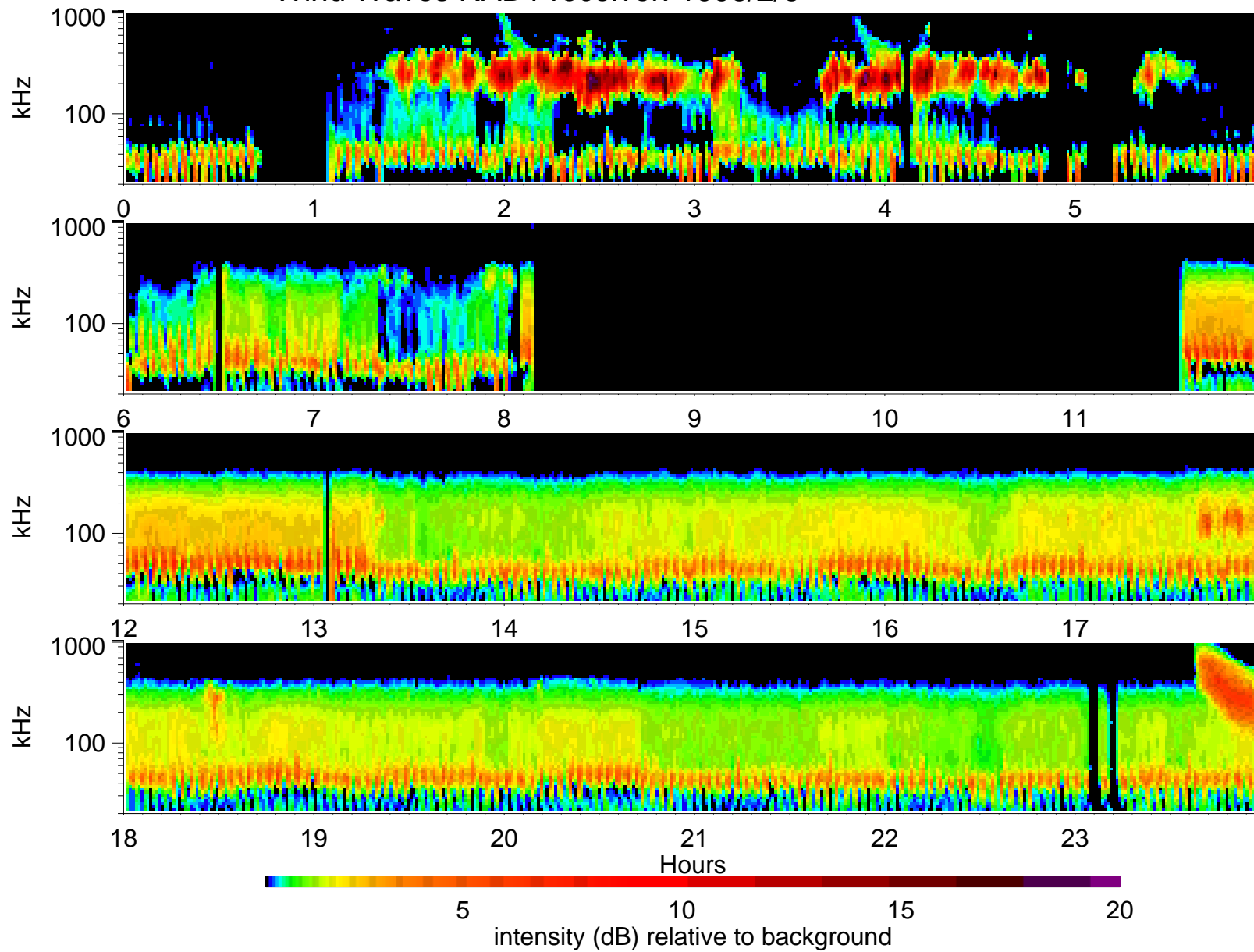
Wind Waves RAD1 receiver: 1998/2/6
