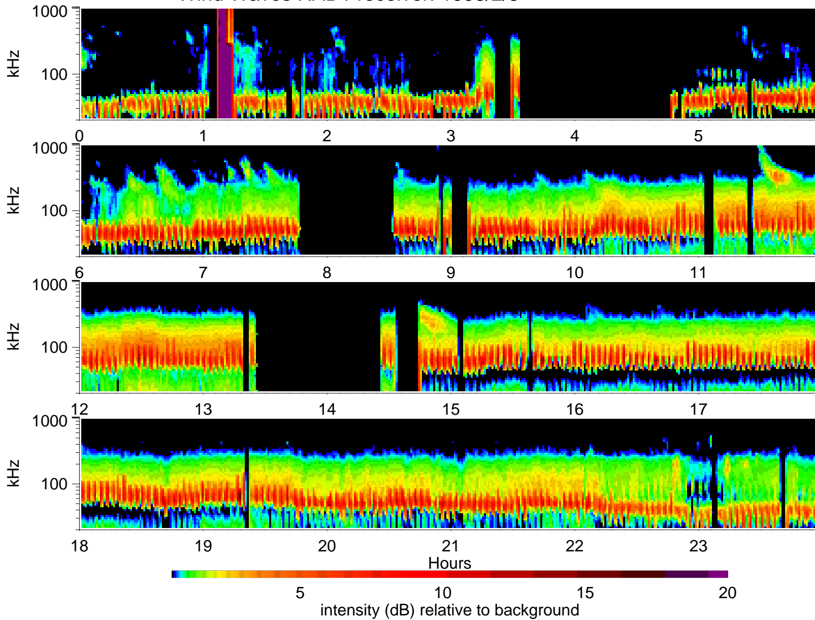
Wind Waves RAD1 receiver: 1998/2/5
