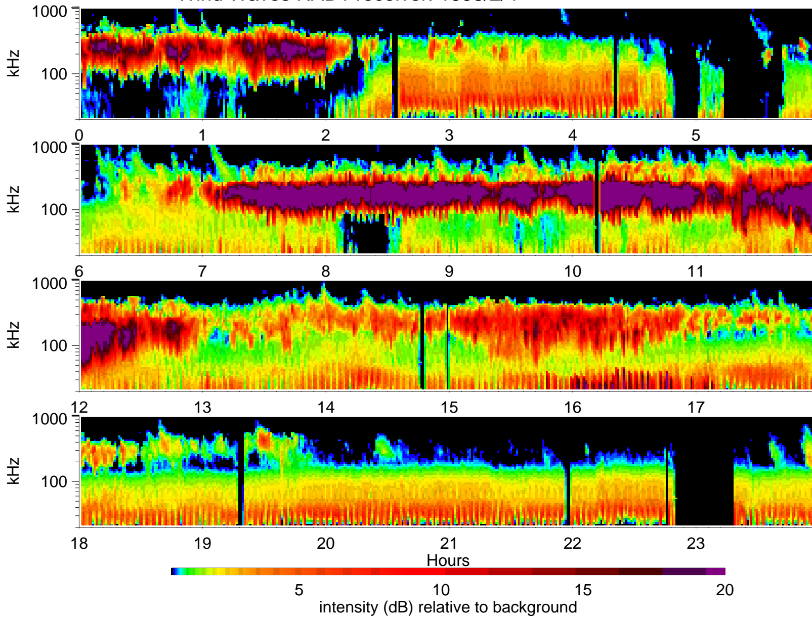
Wind Waves RAD1 receiver: 1998/2/4
