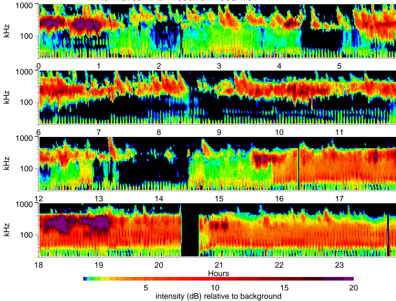
Wind Waves RAD1 receiver: 1998/1/31
