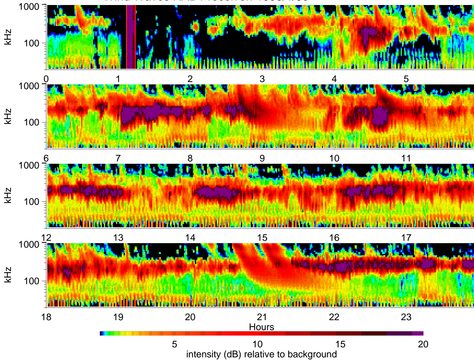
Wind Waves RAD1 receiver: 1998/1/30
