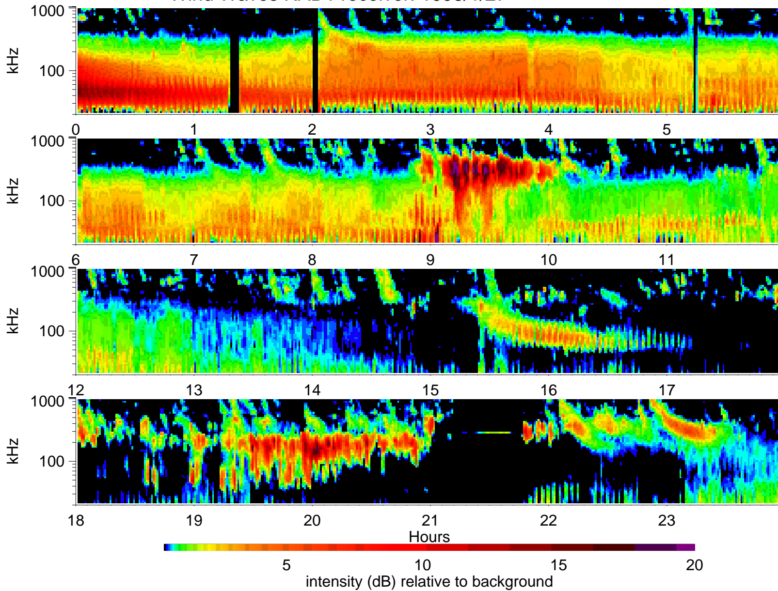
Wind Waves RAD1 receiver: 1998/1/27
