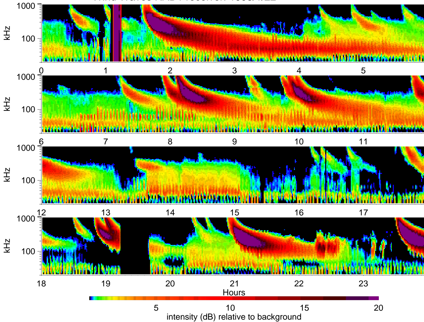
Wind Waves RAD1 receiver: 1998/1/22
