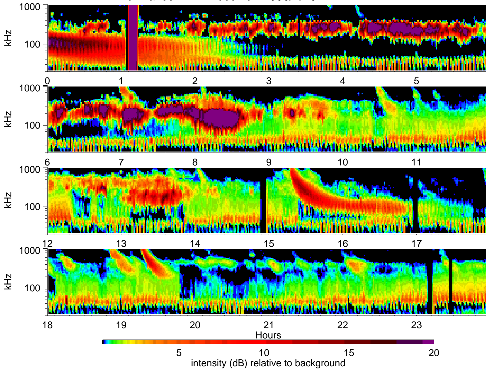
Wind Waves RAD1 receiver: 1998/1/18
