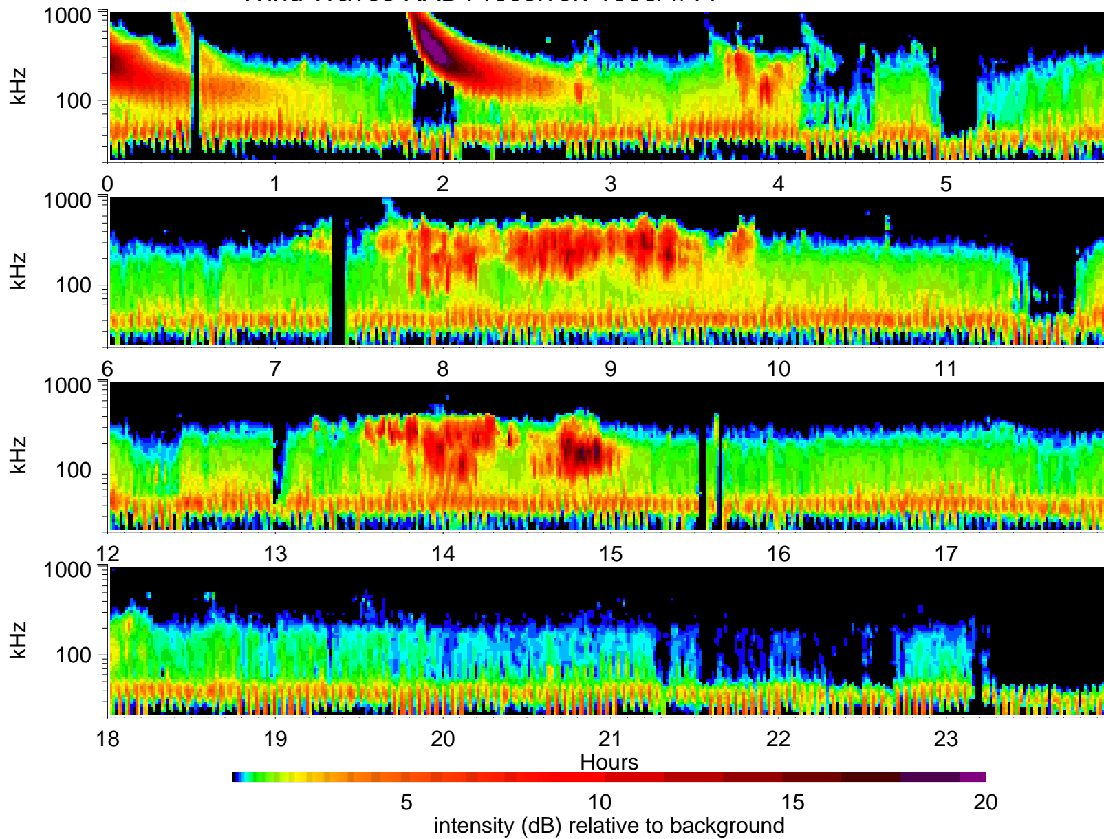
Wind Waves RAD1 receiver: 1998/1/11
