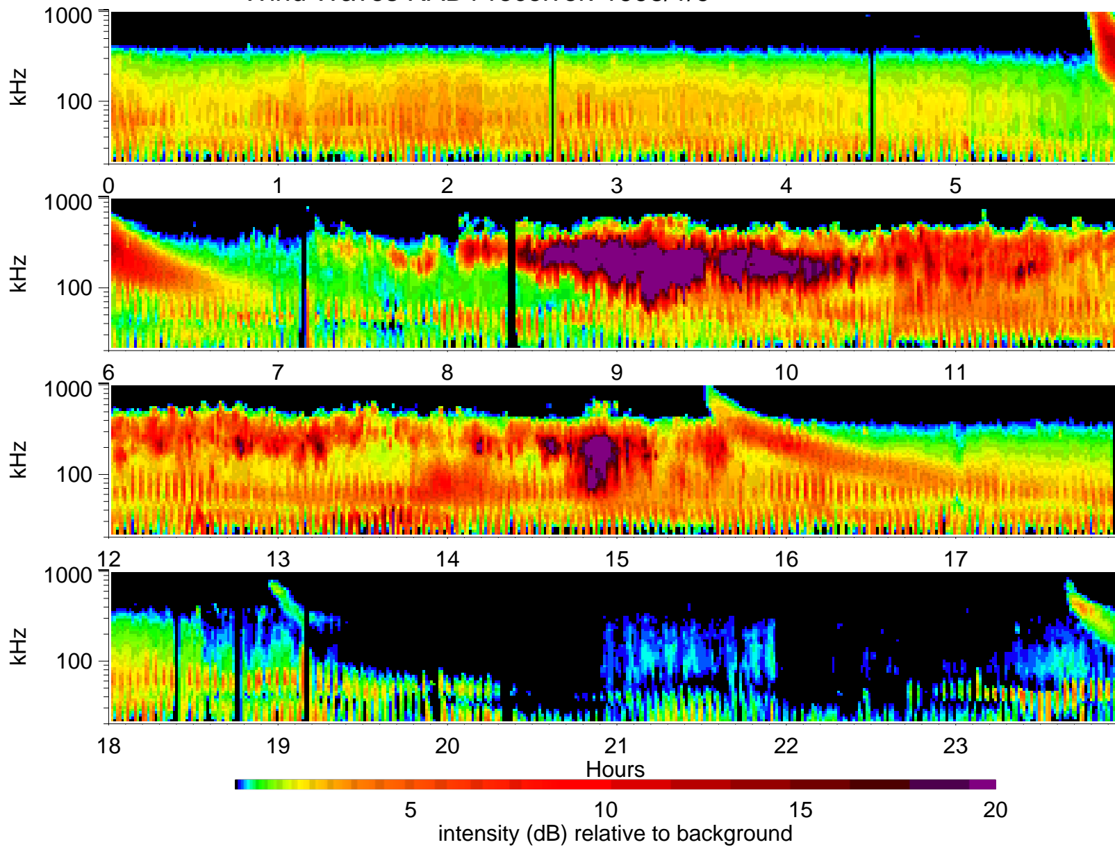
Wind Waves RAD1 receiver: 1998/1/9
