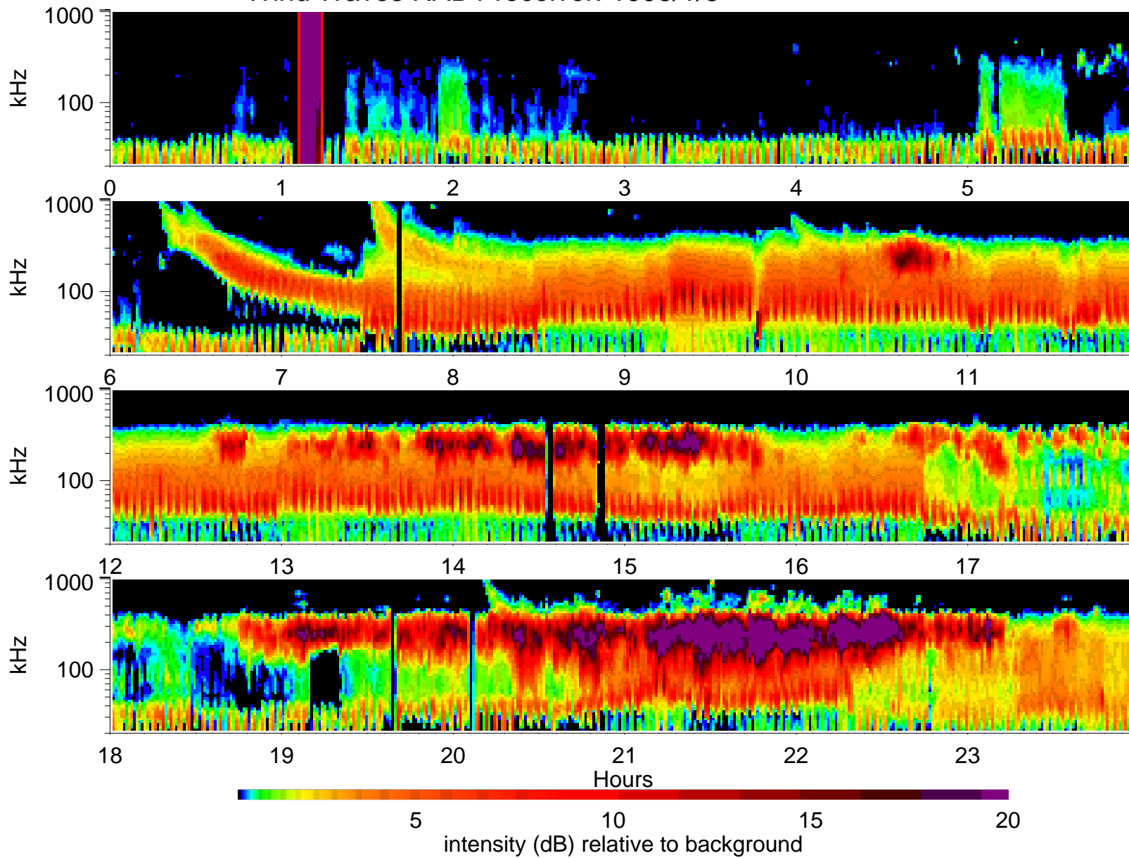
Wind Waves RAD1 receiver: 1998/1/8
