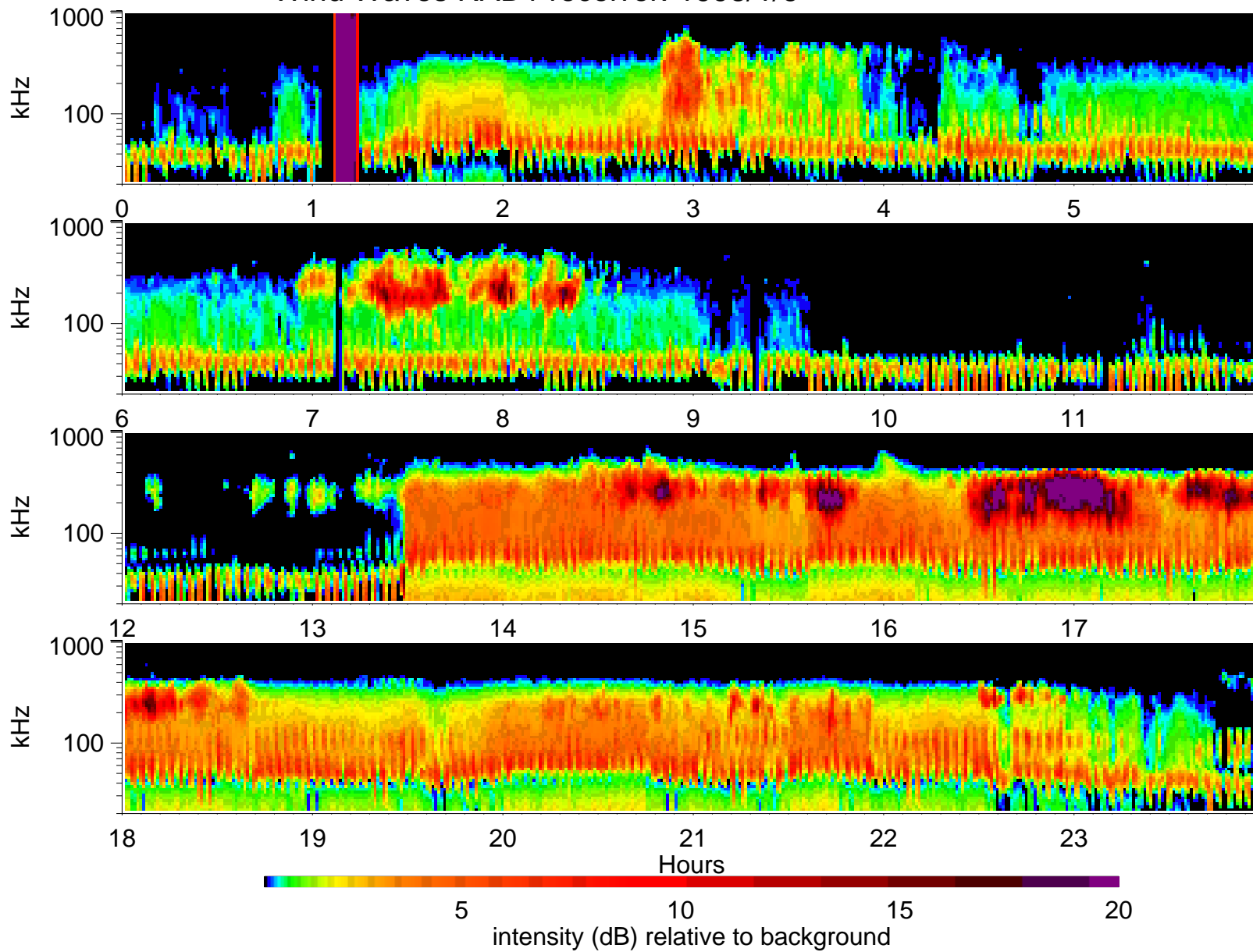
Wind Waves RAD1 receiver: 1998/1/6
