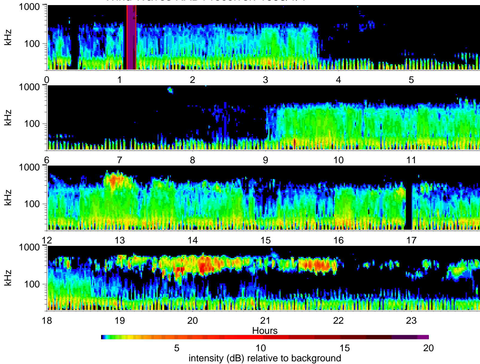
Wind Waves RAD1 receiver: 1998/1/4
