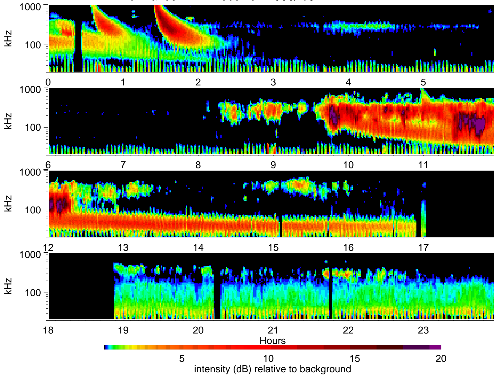
Wind Waves RAD1 receiver: 1998/1/3
