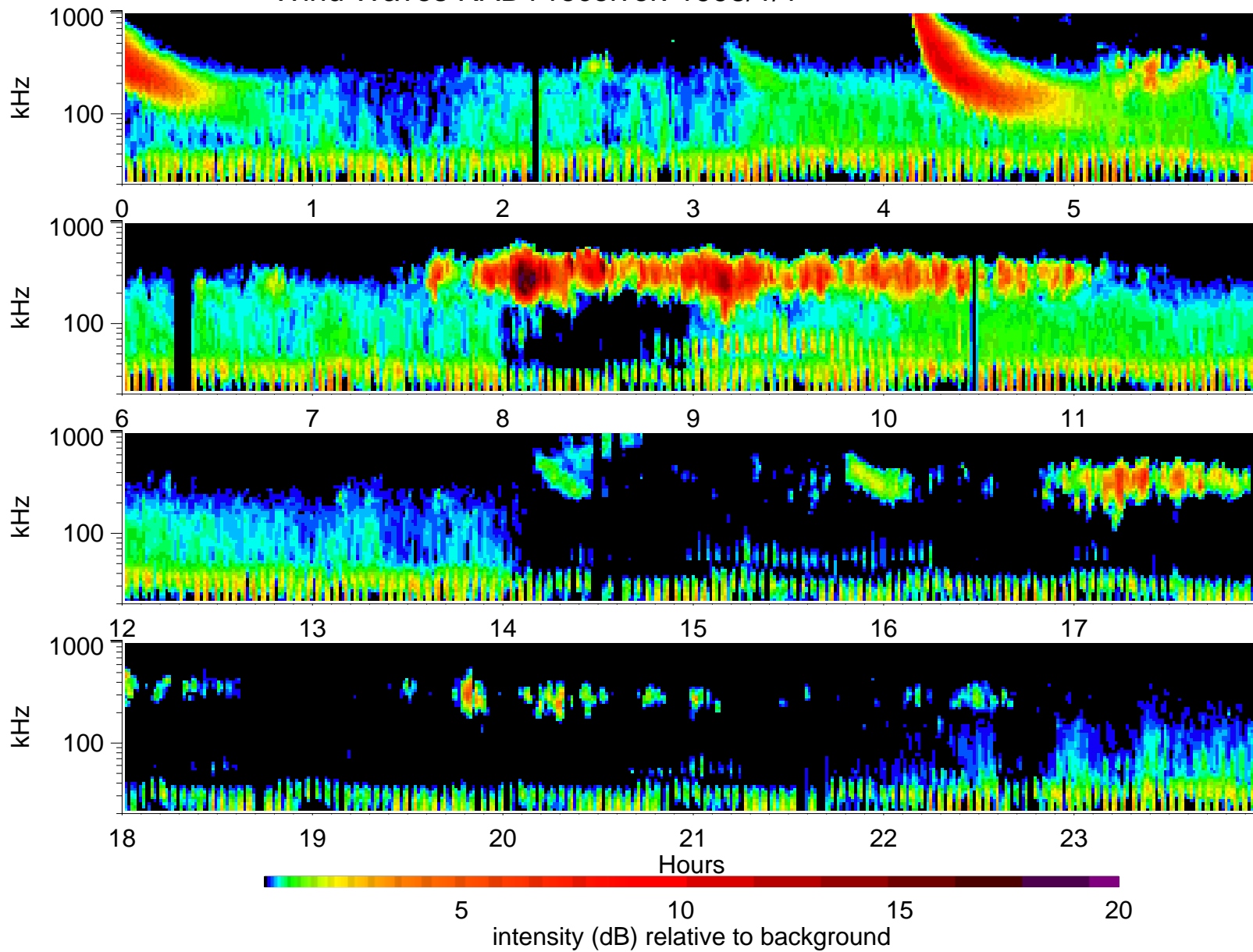
Wind Waves RAD1 receiver: 1998/1/1
