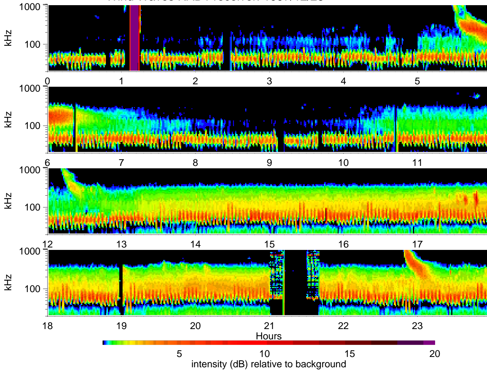
Wind Waves RAD1 receiver: 1997/12/28
