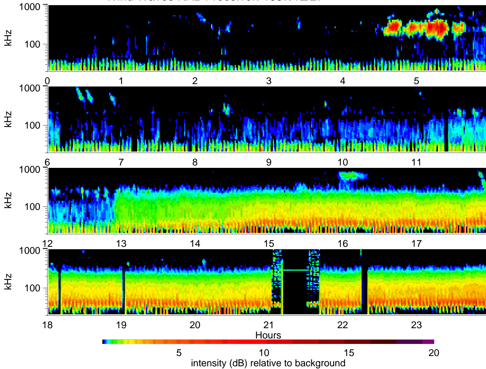
Wind Waves RAD1 receiver: 1997/12/27
