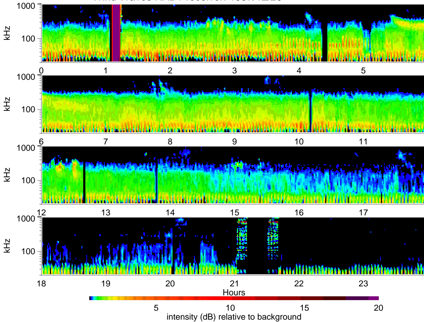
Wind Waves RAD1 receiver: 1997/12/26
