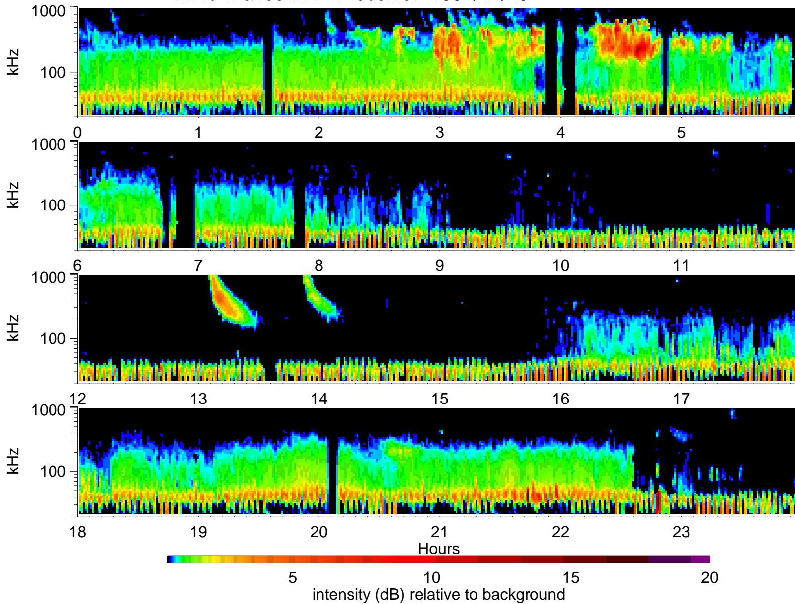
Wind Waves RAD1 receiver: 1997/12/25
