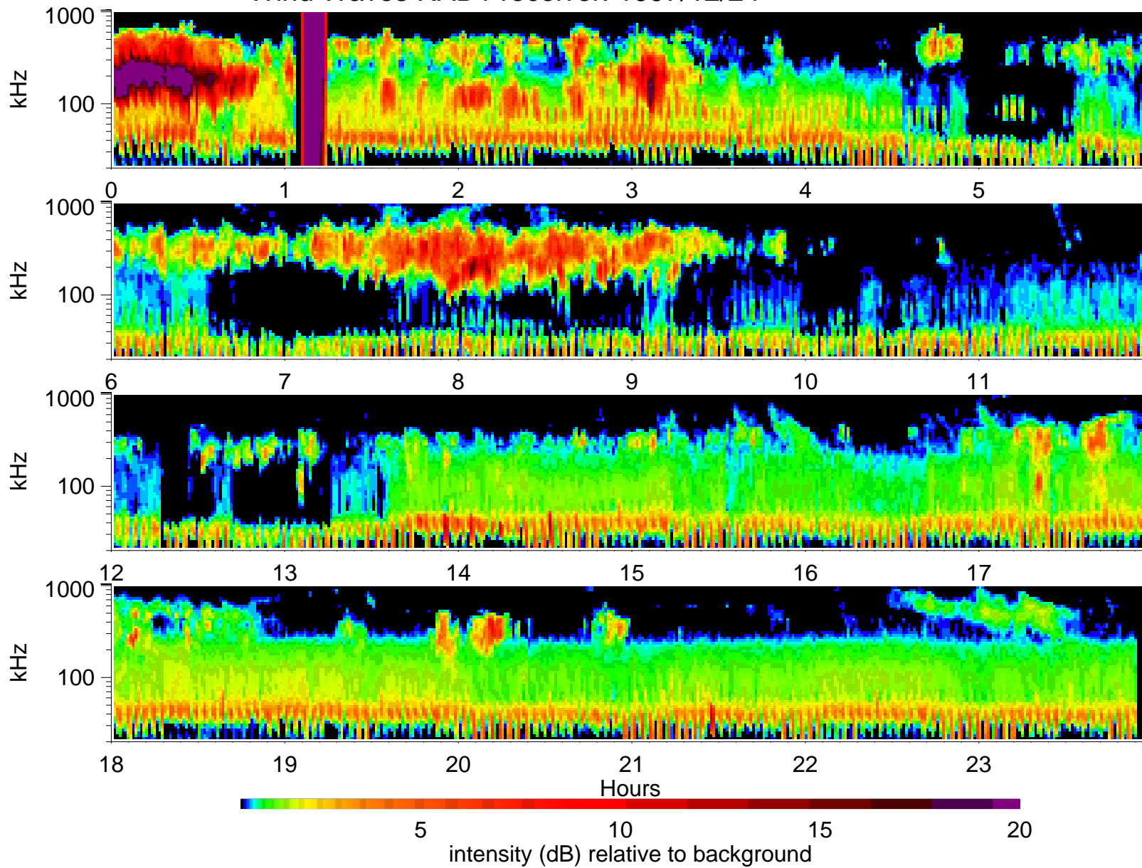
Wind Waves RAD1 receiver: 1997/12/24
