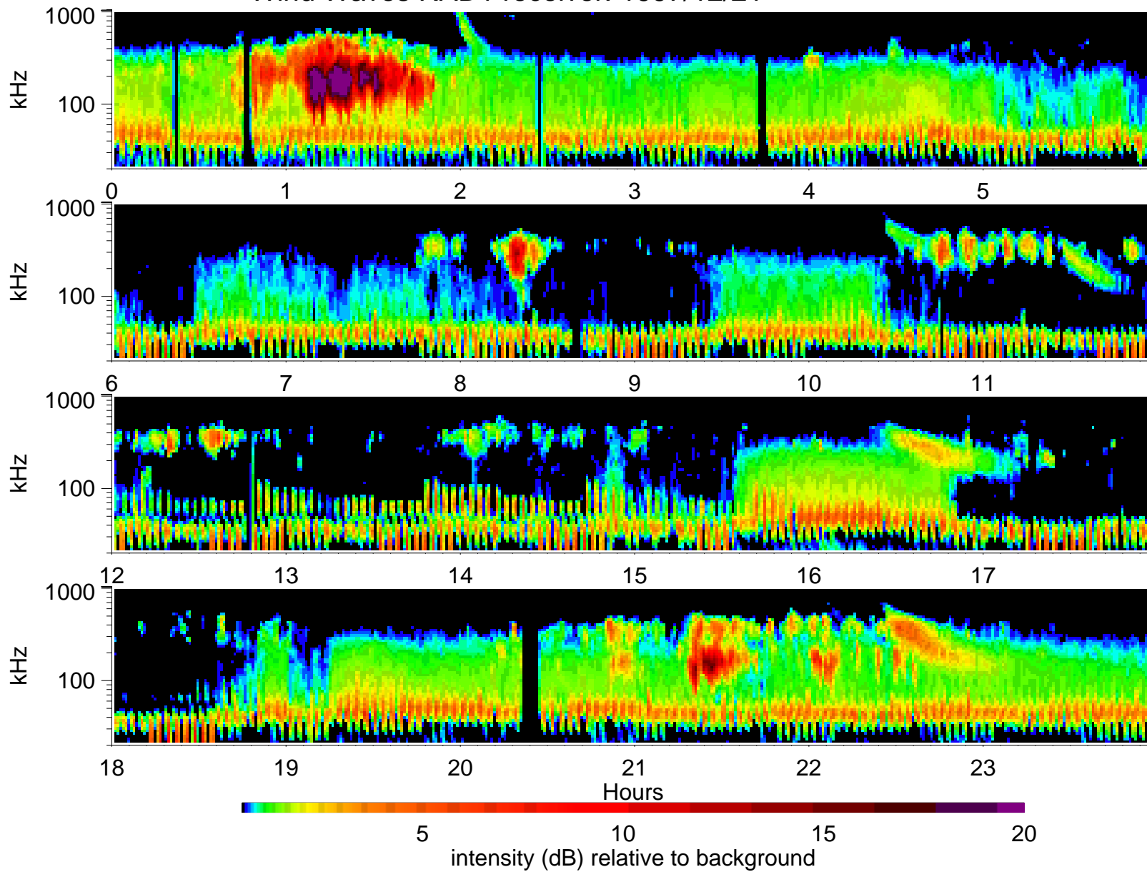
Wind Waves RAD1 receiver: 1997/12/21
