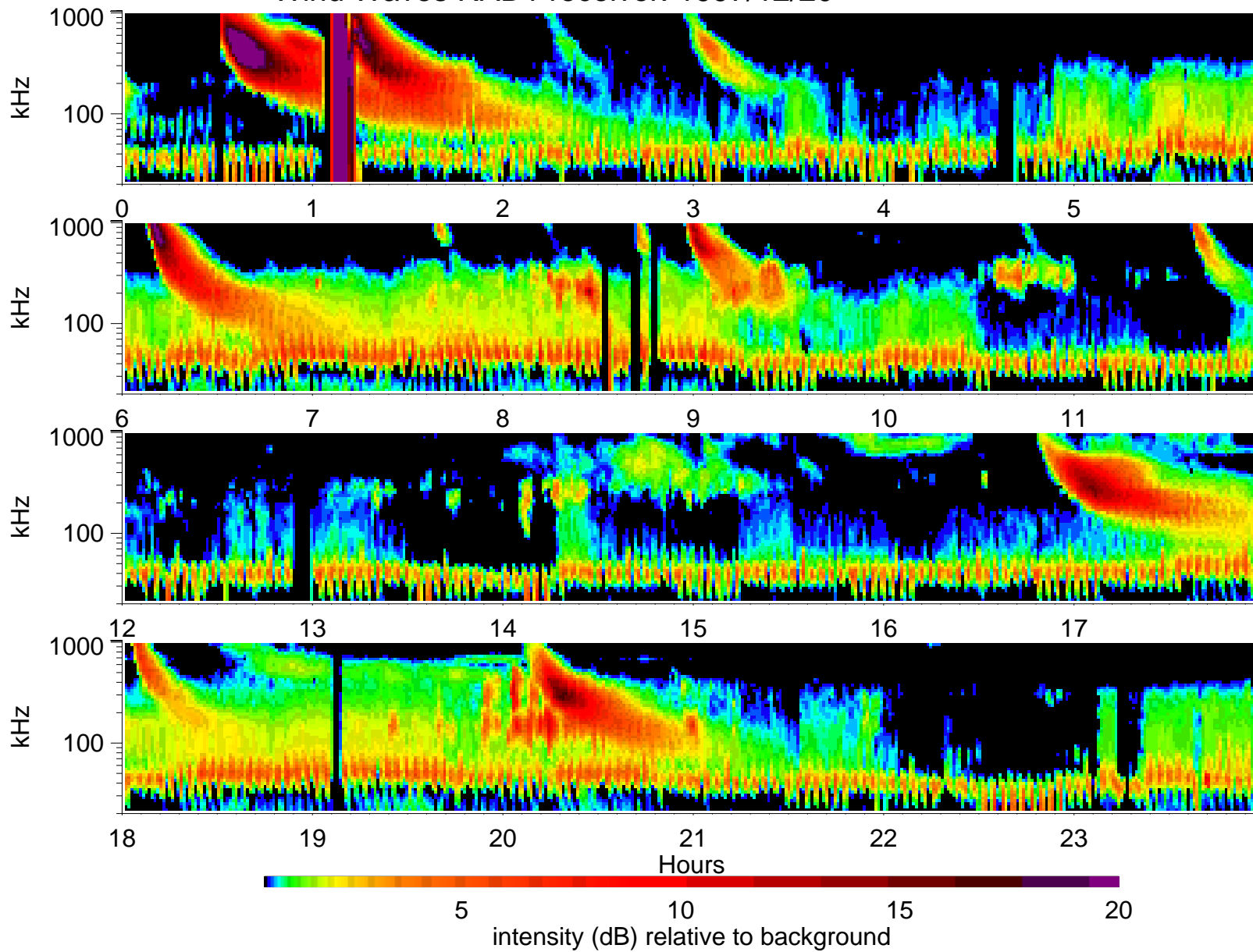
Wind Waves RAD1 receiver: 1997/12/20
