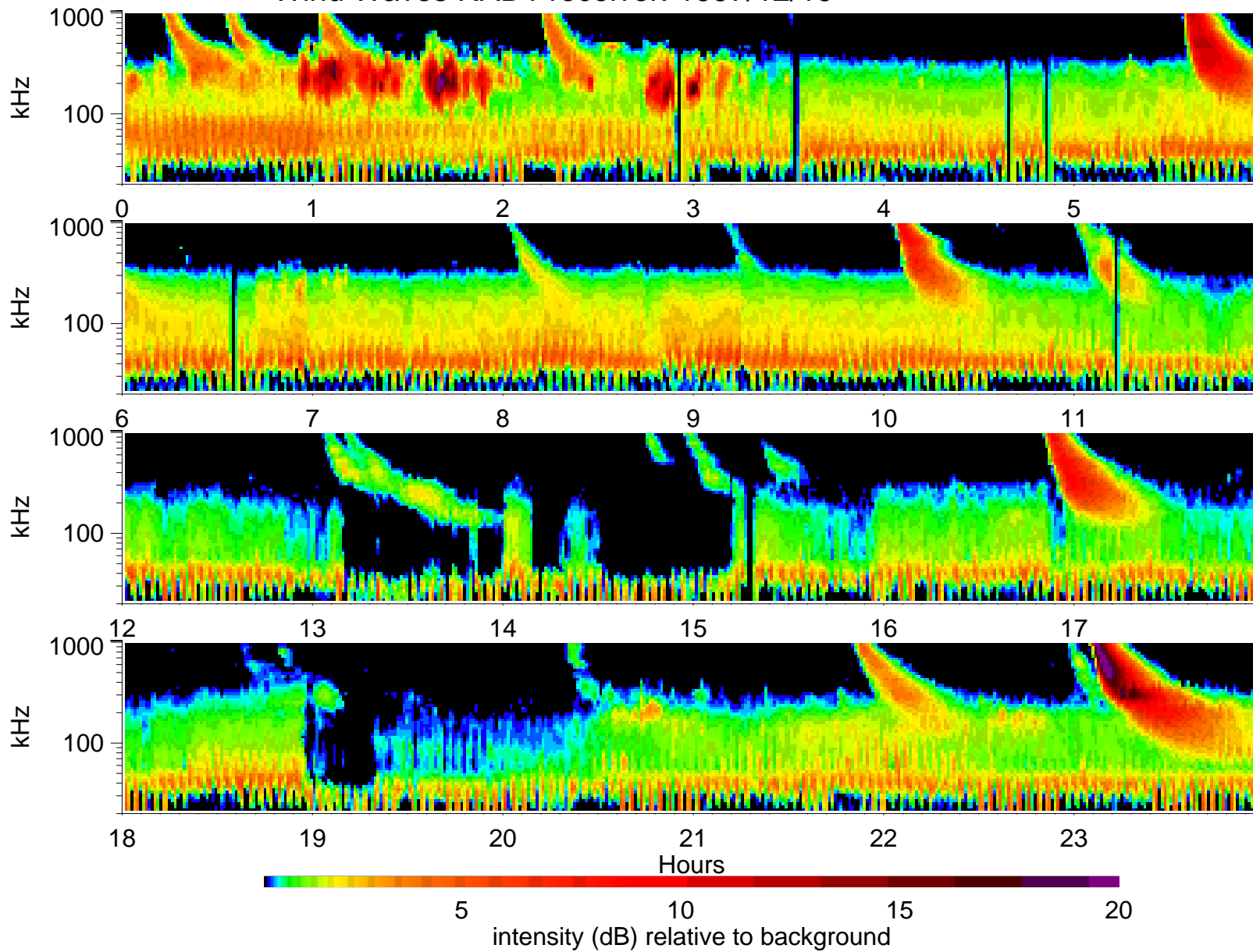
Wind Waves RAD1 receiver: 1997/12/19
