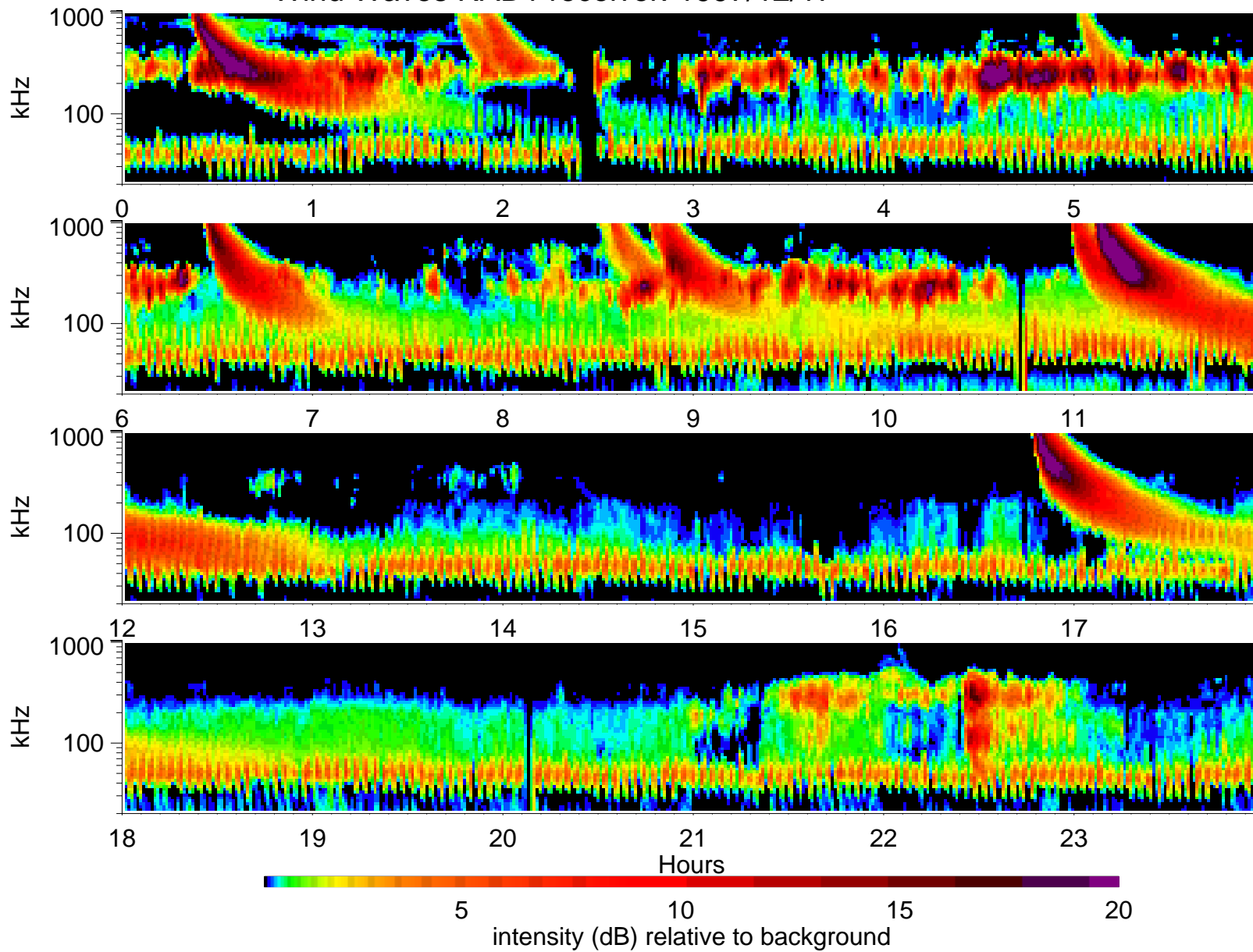
Wind Waves RAD1 receiver: 1997/12/17
