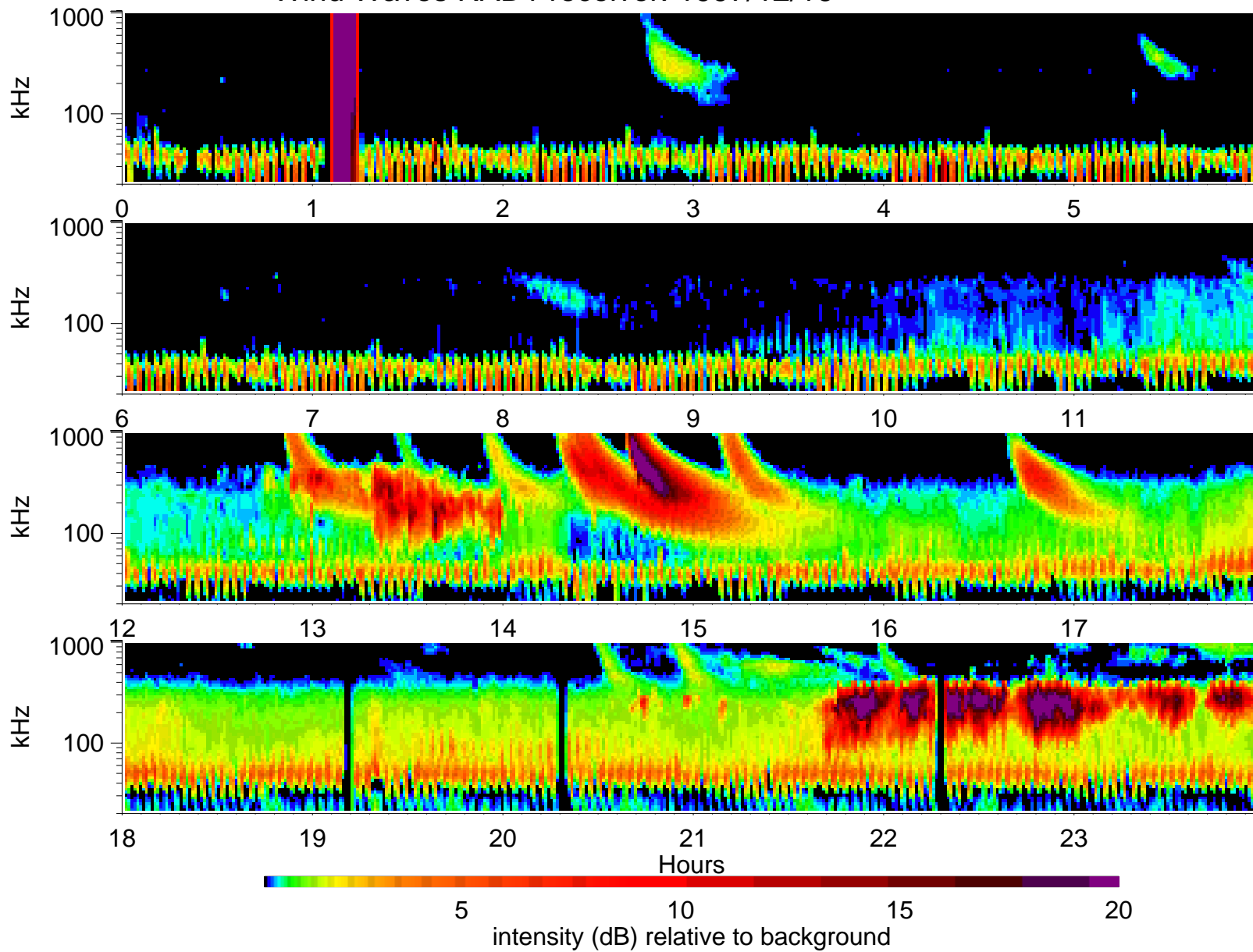
Wind Waves RAD1 receiver: 1997/12/16
