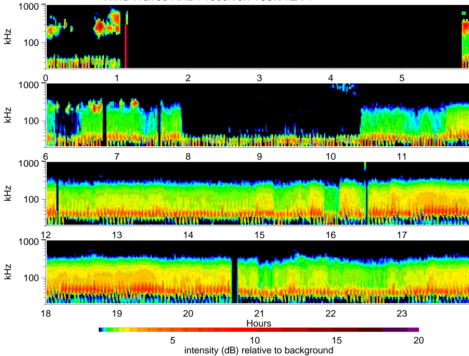
Wind Waves RAD1 receiver: 1997/12/14
