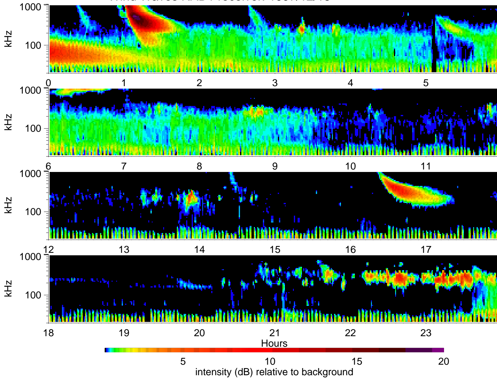
Wind Waves RAD1 receiver: 1997/12/13
