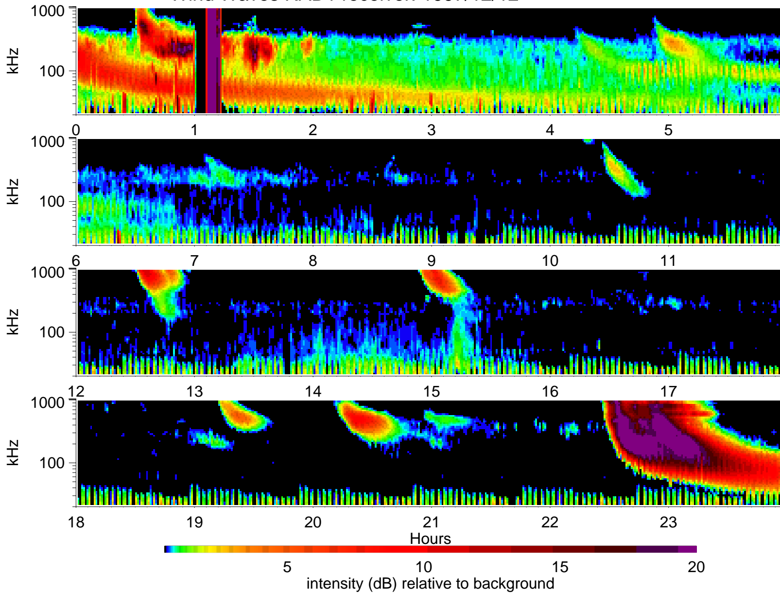
Wind Waves RAD1 receiver: 1997/12/12
