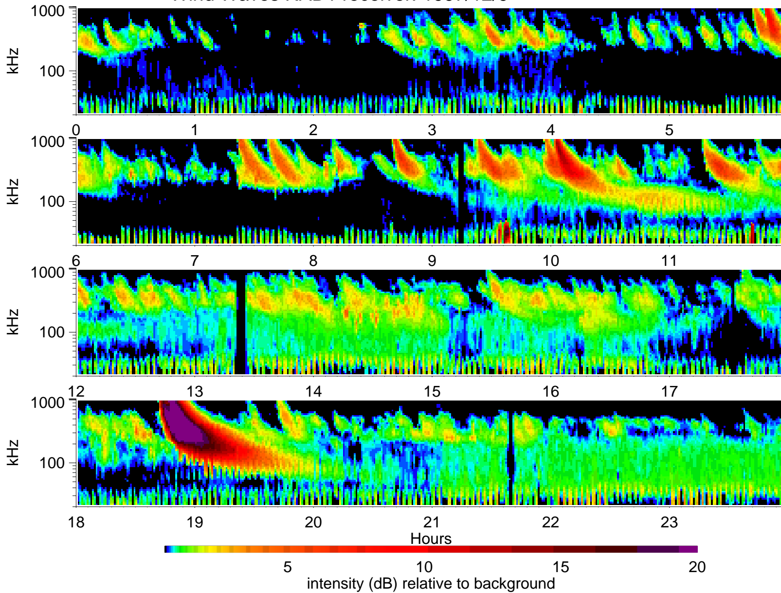
Wind Waves RAD1 receiver: 1997/12/9
