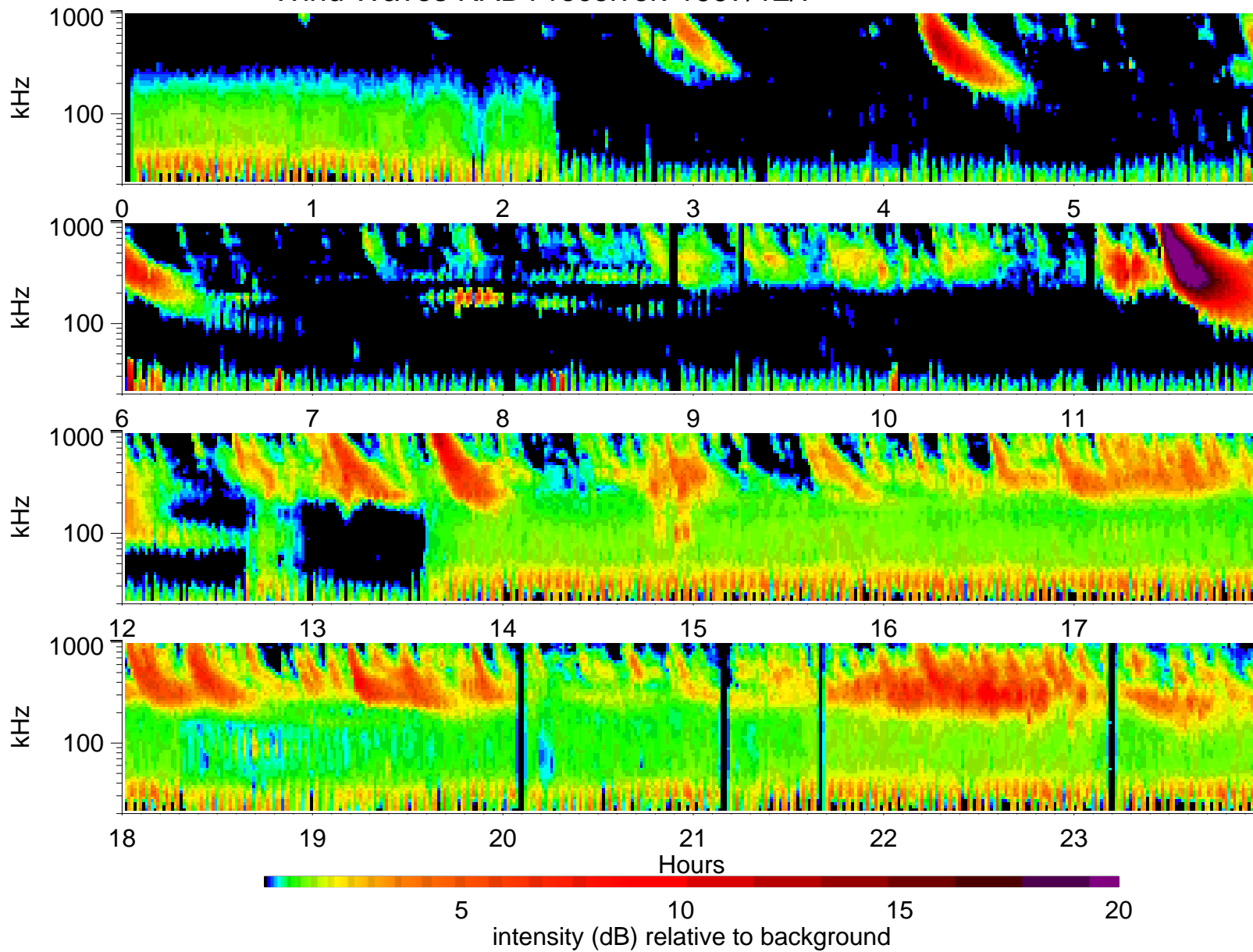
Wind Waves RAD1 receiver: 1997/12/7
