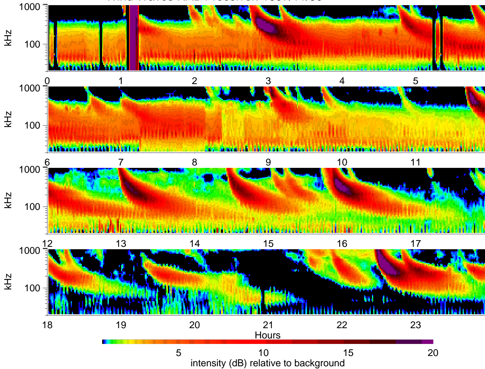
Wind Waves RAD1 receiver: 1997/11/30
