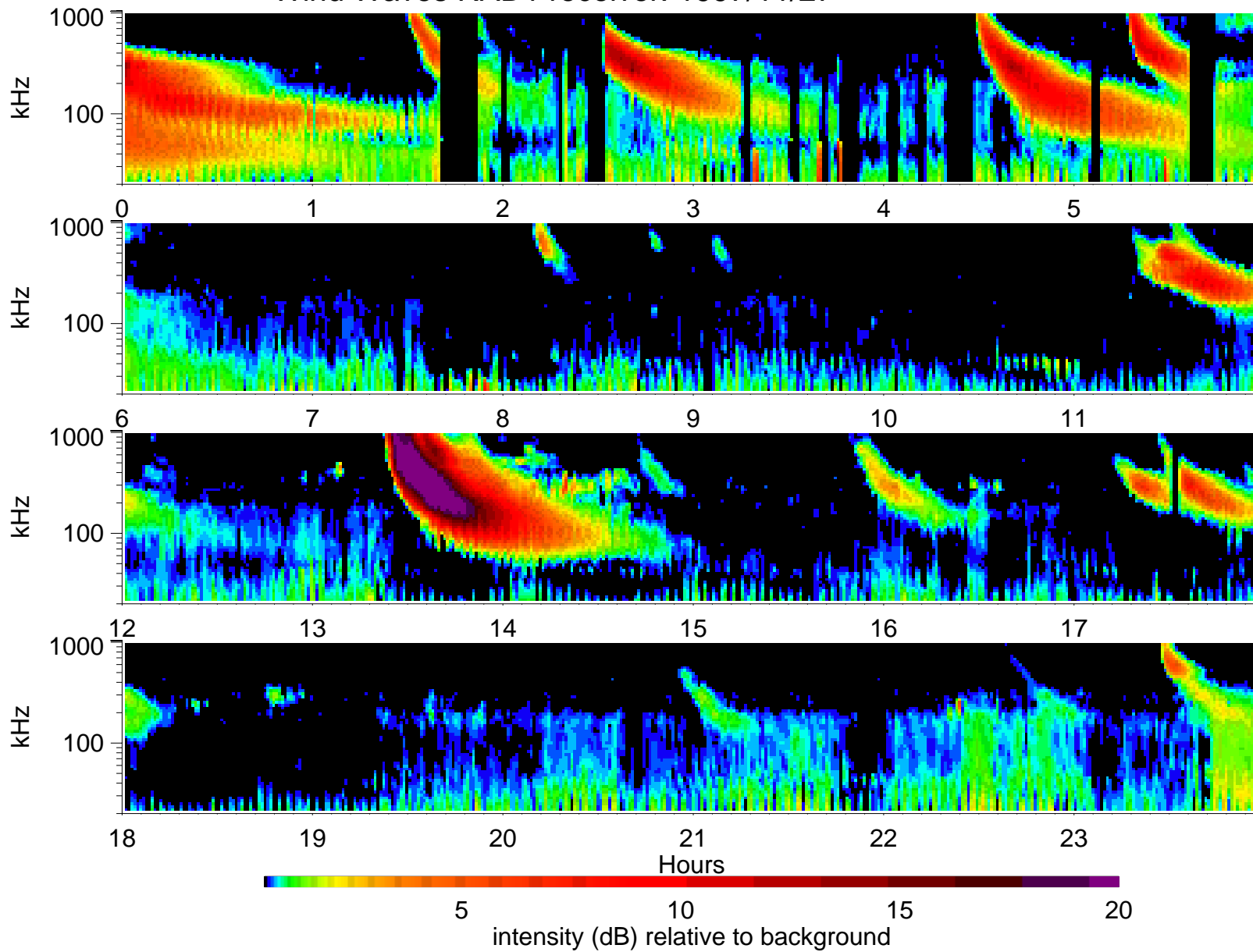
Wind Waves RAD1 receiver: 1997/11/27
