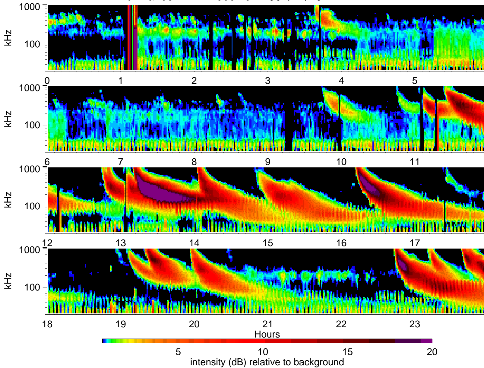
Wind Waves RAD1 receiver: 1997/11/26
