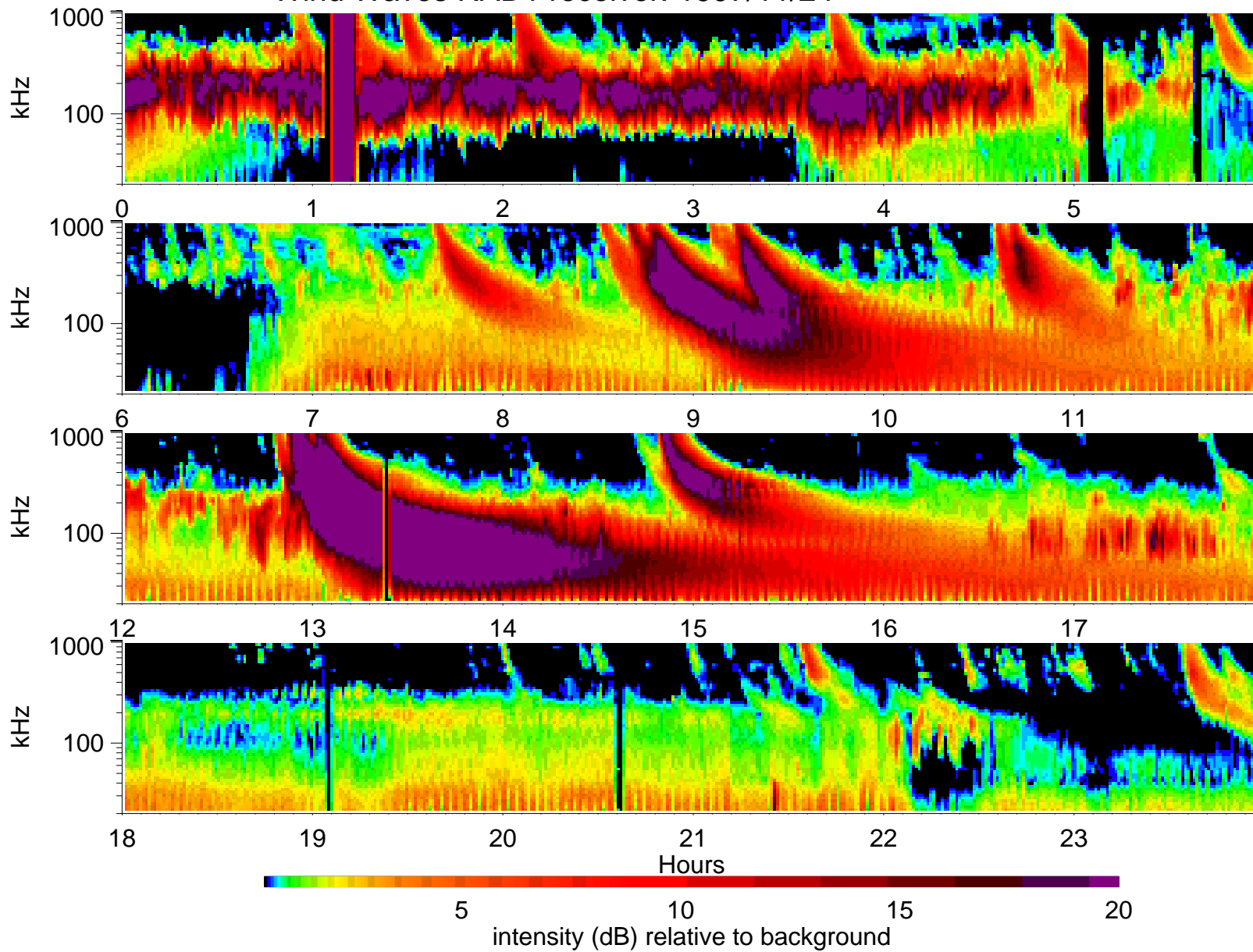
Wind Waves RAD1 receiver: 1997/11/24
