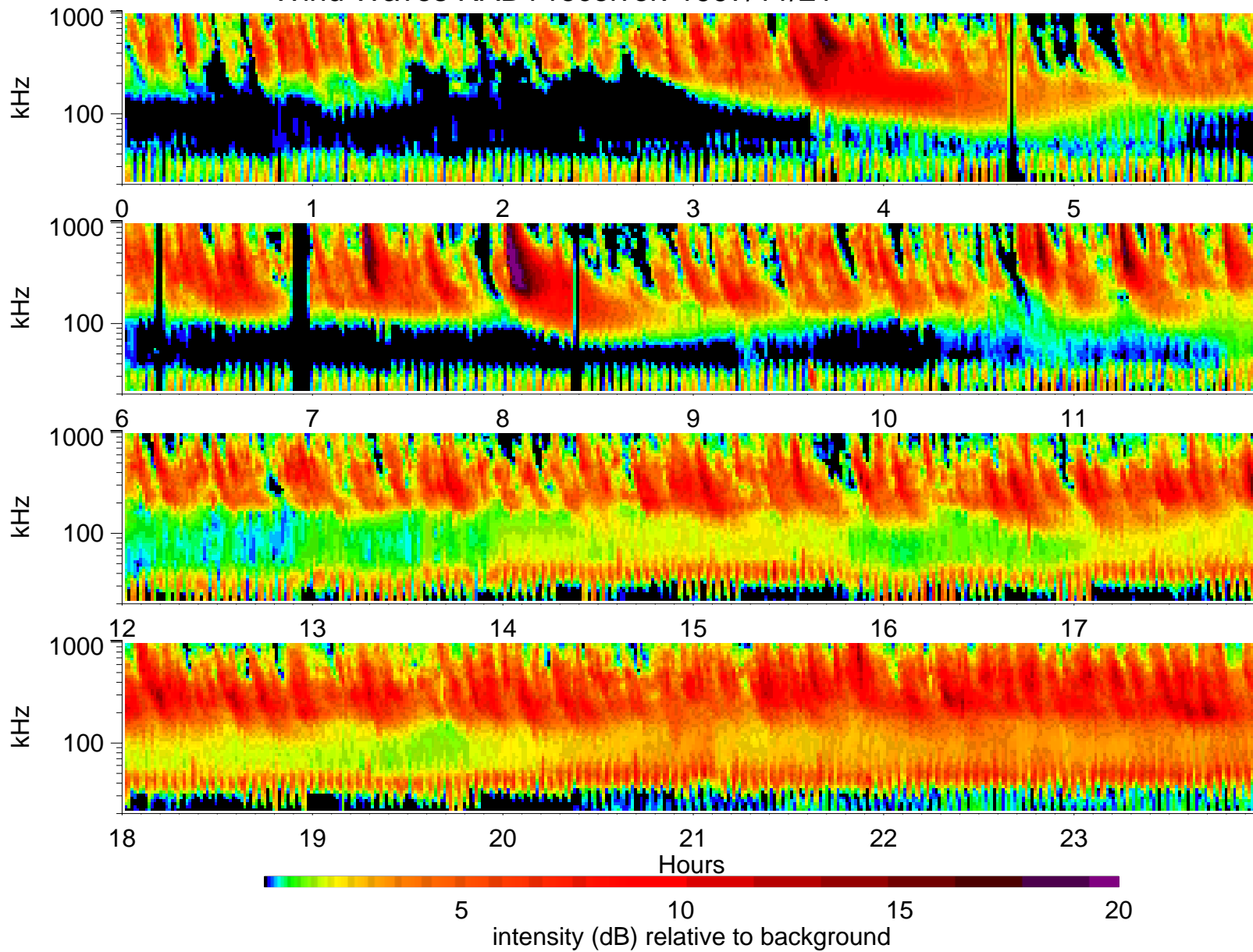
Wind Waves RAD1 receiver: 1997/11/21
